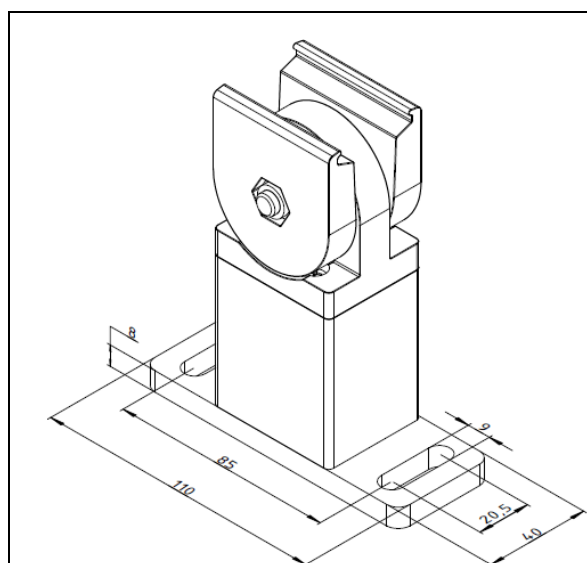
3. Guide rail bracket (Type A)
