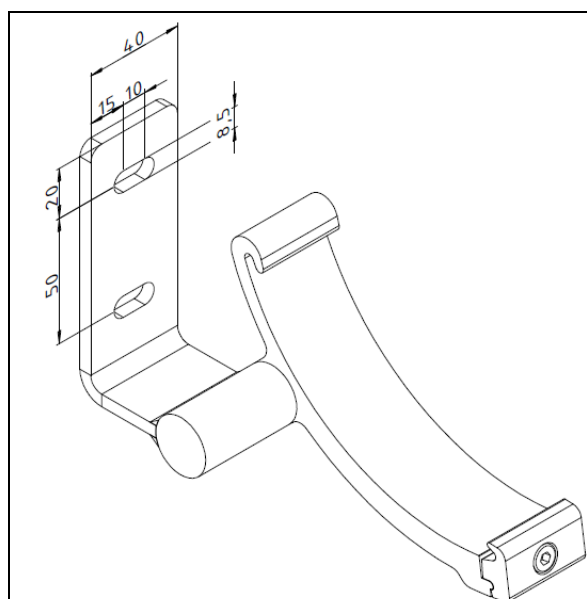
1. Vertical cassette bracket
