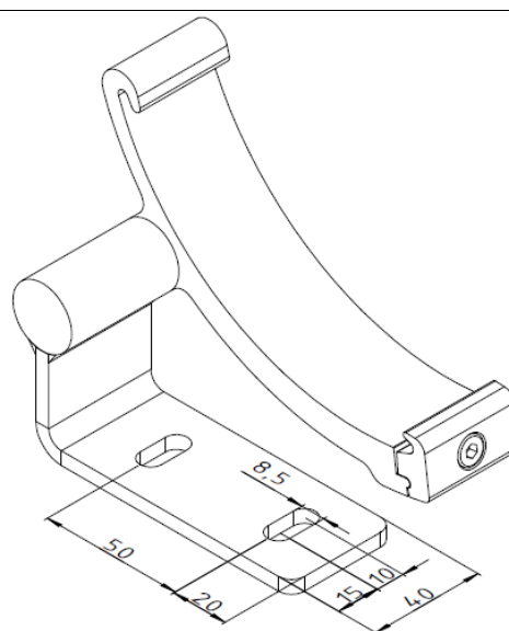
2. Horizontal cassette bracket
