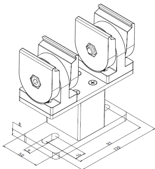
7. Modular transverse guide rail bracket (Type G)
