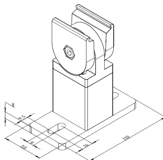
4. Transverse guide rail bracket (Type D)
